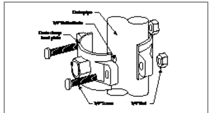
Drain saddle valve installation (from front)
